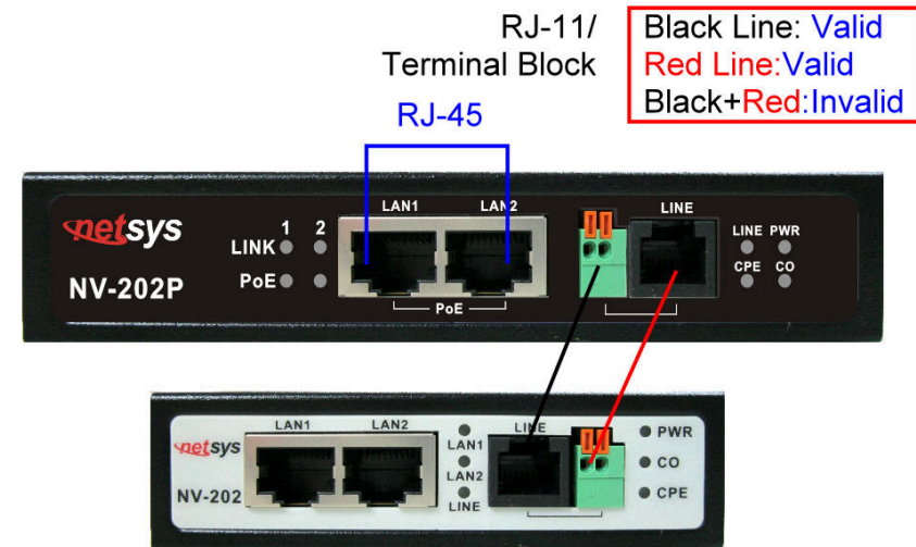
Figure 2.5 NV-202P line ports crossover connection
