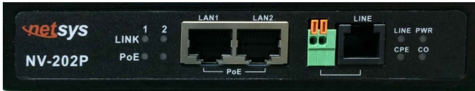
Figure 3.1 Front Panel
