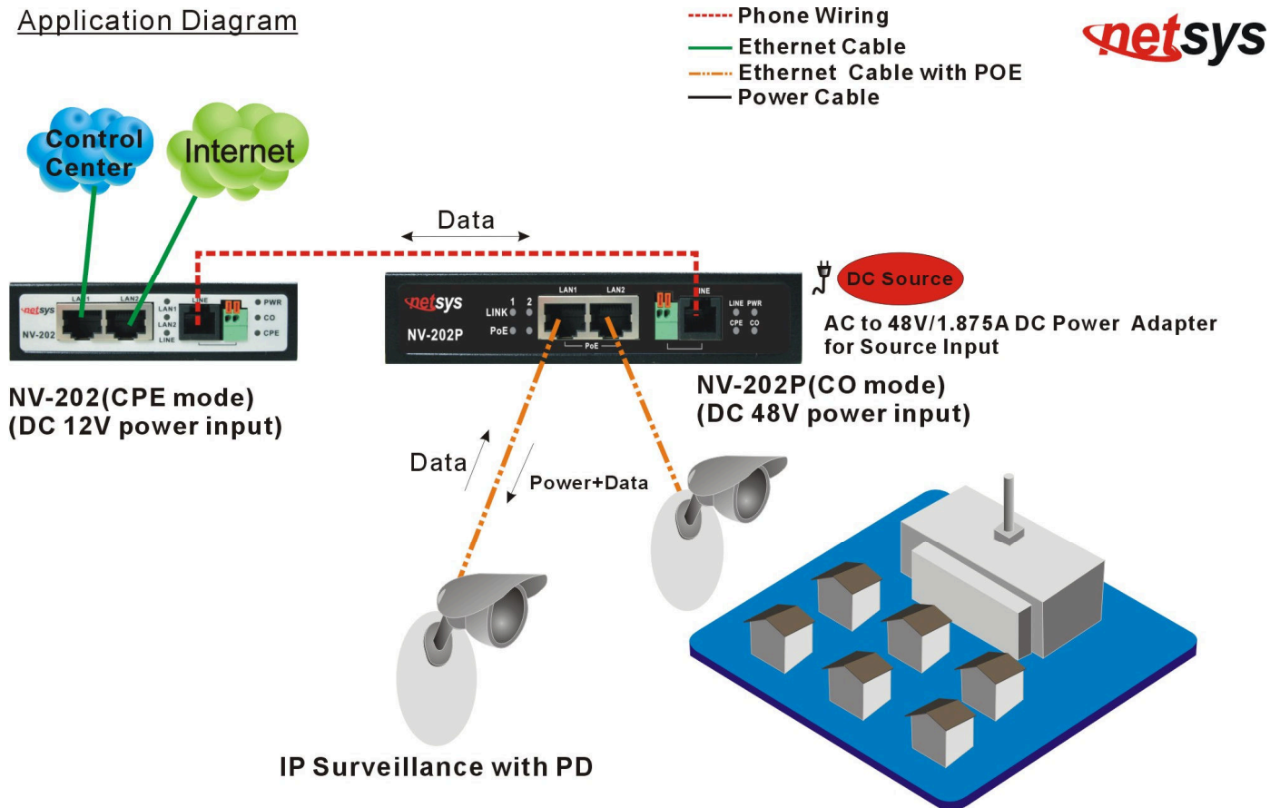
Figure 2.7 NV-202 / NV-202P point to point application diagram
