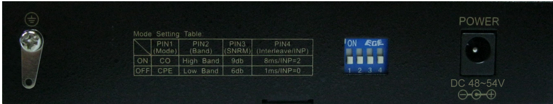
Figure 3.2 Rear Panel
